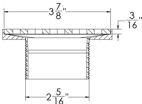
SECTION 1-1
