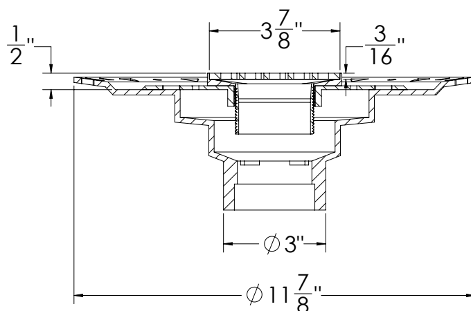
SECTION 1-1
