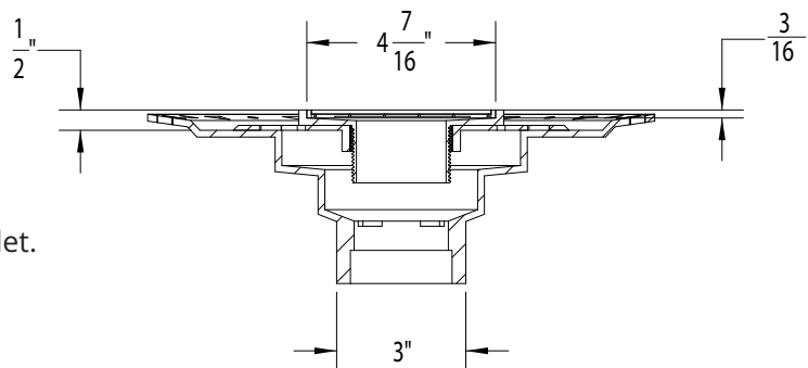
SECTION 1-1
