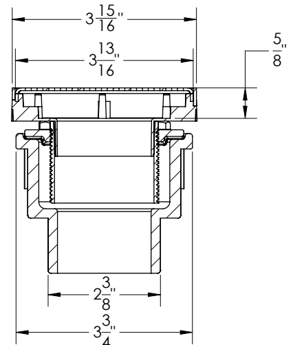
SECTION 1-1
