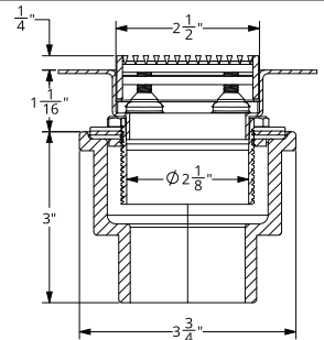
Section View
