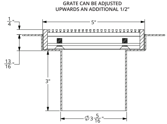
SECTION 1-1
