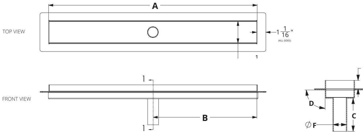
SECTION 1-1
