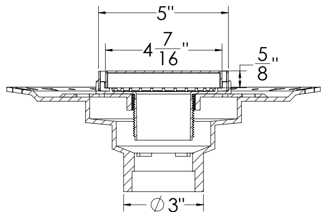
SECTION 1-1
