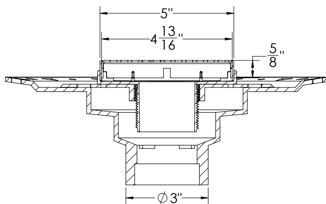
SECTION 1-1
