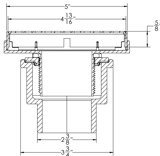
SECTION 1-1
