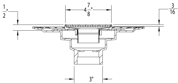
SECTION 1-1
