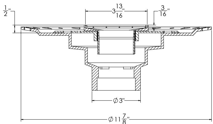
SECTION 1-1
