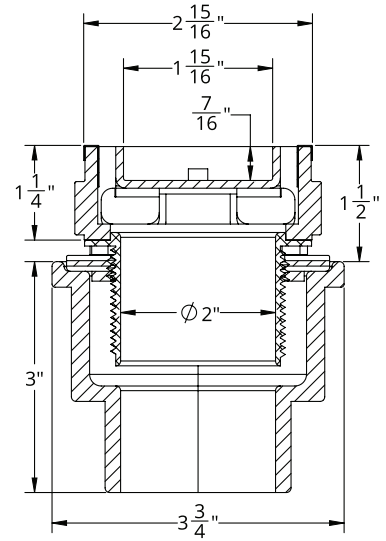
SECTION 1-1
