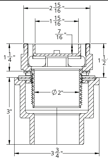
SECTION 1-1
