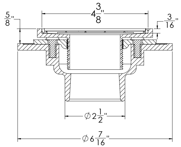
SECTION 1-1
