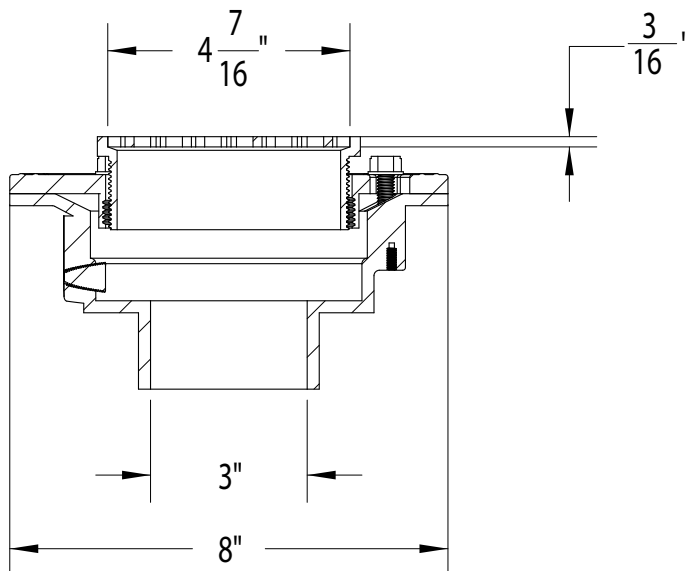
SECTION 1-1
