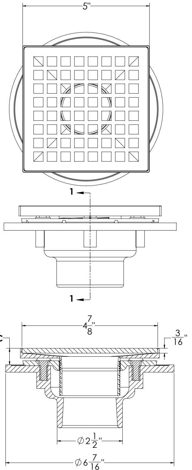
SECTION 1-1
