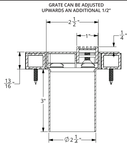
SECTION 1-1
