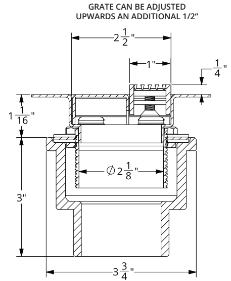
SECTION 1-1
