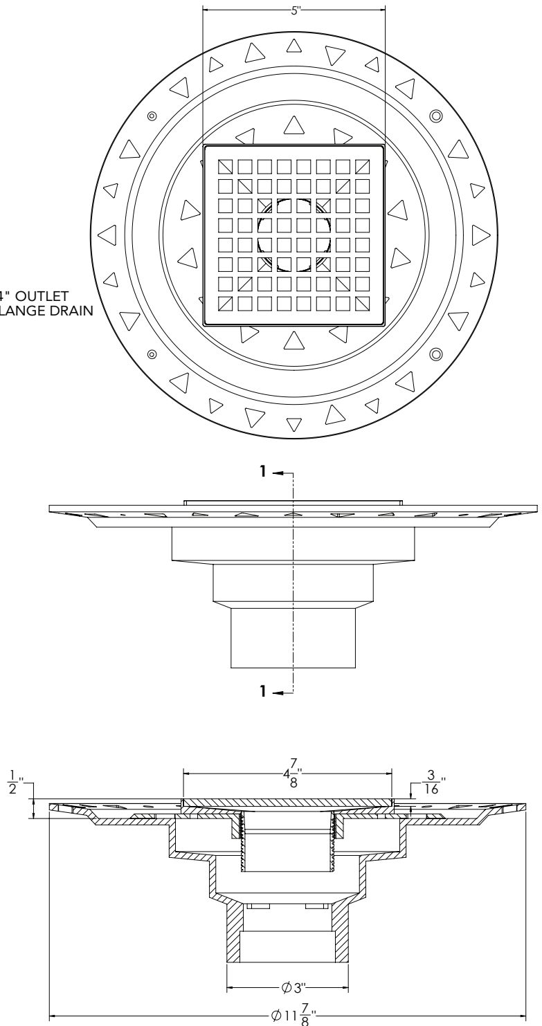
SECTION 1-1
