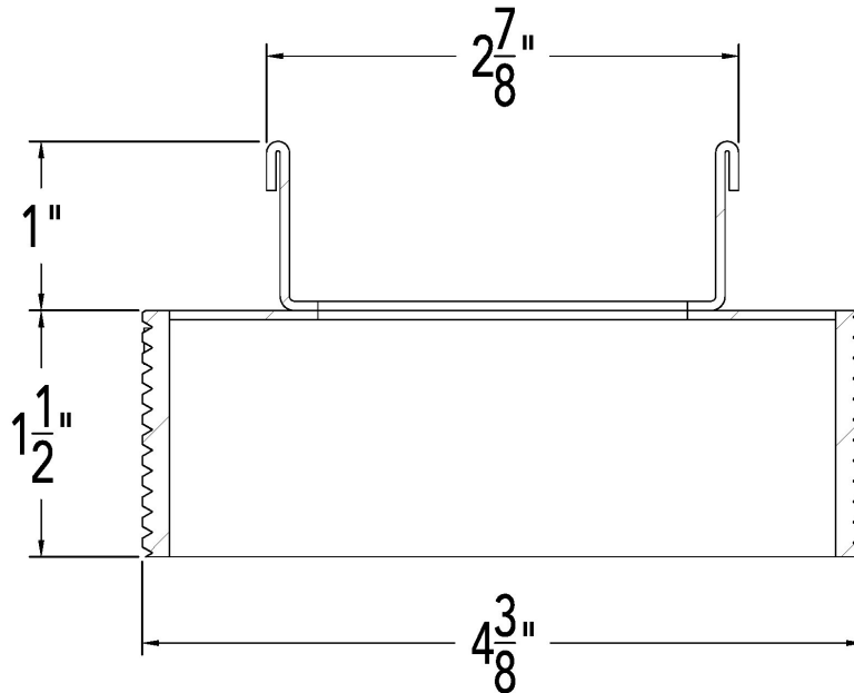
8" Stainless steel outlet assembly for S-DGAS/AS 99 Series w/ 4" threaded nipple attached
