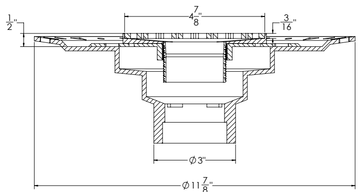
SECTION 1-1
