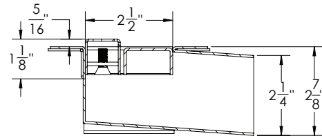
SECTION 1-1
