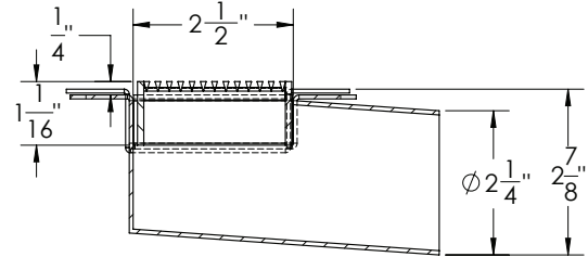
SECTION 1-1
