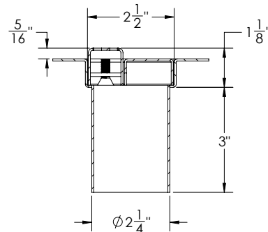
SECTION 1-1
